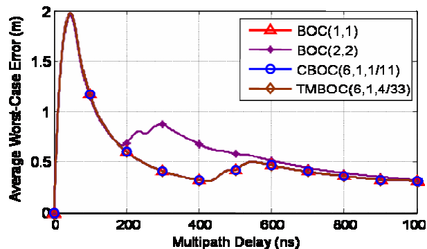
Fig. 14. Average Error for Double-Delta Processing, BW=24 MHz (4 pole Butterworth filter), Early-Late Spacings of 24.4 nsec and 48.9 nsec
