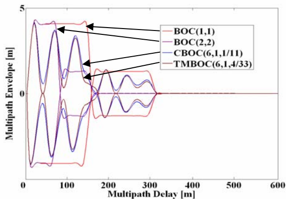
Fig. 9. Multipath Error Envelope for NELP Processing, BW=24 MHz (6 pole Butterworth filter), d=0.05 chips
