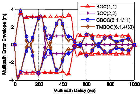
Fig. 5. Multipath Error Envelope for NELP Processing, BW=24 MHz (4 pole Butterworth), \Delta\tau=24.4 nsec
