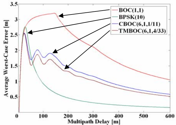
Fig. 8. Average Error for NELP Processing, BW=24 MHz (6 pole Butterworth filter), d=0.0125 chips
