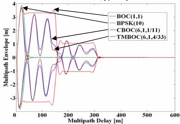
Fig. 7. Multipath Error Envelope for NELP Processing, W=24 MHz (6 pole Butterworth filter), d=0.0125 chips
