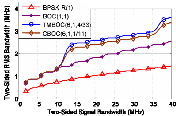
Fig. 15. RMS bandwidth vs. two-sided receiver bandwidth
