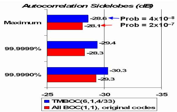
Fig. 17. Comparison of L1C Autocorrelation Sidelobes
