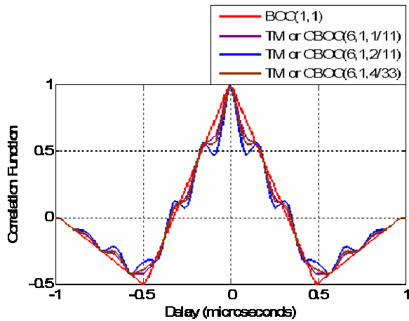
Fig. 4. Normalized Autocorrelation Functions Computed over \pm 15 MHz Bandwidth Summary of Spreading Time Series and Implementation
