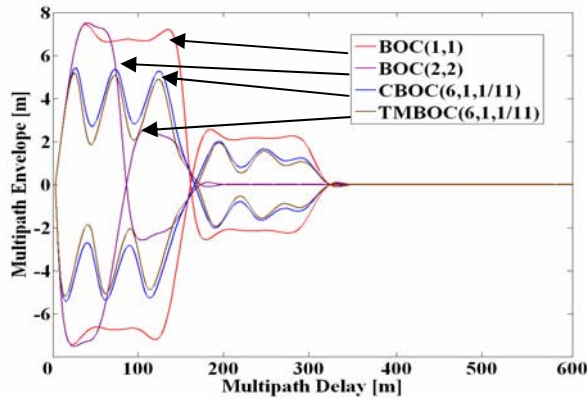
Fig. 11. Multipath Error Envelope for NELP Processing, BW=12 MHz (6 pole Butterworth filter), d=0.05 chips
