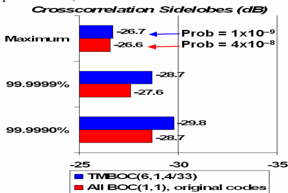
Fig. 16. Comparison of L1C Crosscorrelation Sidelobes
