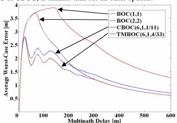
Fig. 10. Average Error for NELP Processing, BW=24 MHz (6 pole Butterworth filter), d=0.05 chips
